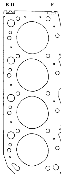
GRADE NOTCHES
